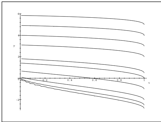
Figure 2: Optimal stopping curve u(t) for d = -2.8, \dots, d = 5
