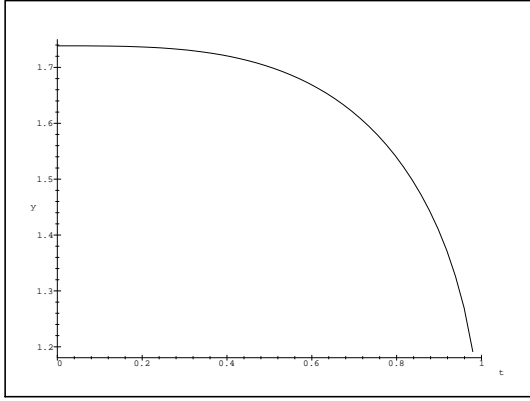
Figure 1: Optimal stopping boundary u(t) , \alpha = 2, c = 1, d = 1
